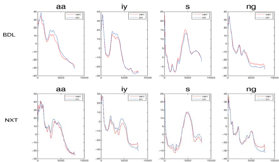
Figure 3: Comparing mean FFT spectra of different phonemes for English speakers BDL and NXT. (blue is speech in noise, red is speech without noise)
