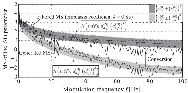
Fig. 7. An example of the MS conversion in the synthesis stage. Note that the MS envelope (“Generated MS” and “Filtered MS”) is drawn instead of the MS itself for clear illustration. The MS envelope is calculated by low-pass lifting the cepstrum of MS.
