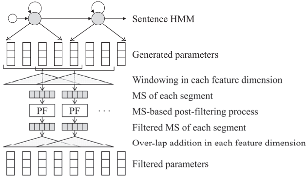
Fig. 9. Procedures of the segment-level MS-based post-filter in HMM-based TTS.
