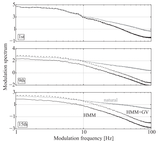
Fig. 3. Averaged MSs of the 1st, 9th and 15th mel-cepstral coefficient sequences from above in HMM-based TTS.
