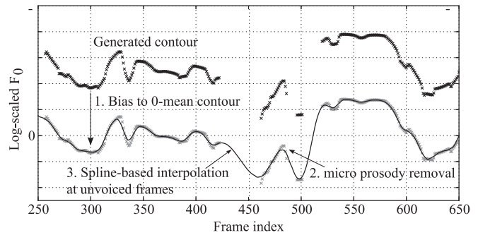
Fig. 8. An illustration of the pre-processing procedures to calculate the continuous F_0 contour from the original F_0 contour.
