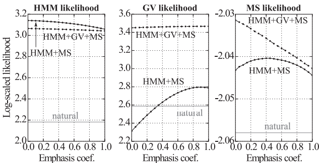
Fig. 19. HMM, GV, and MS likelihoods for the F_0 contours filtered by the proposed segment-level post-filter in HMM-based TTS.
