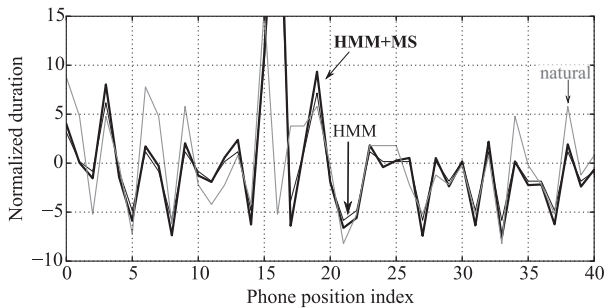
Fig. 13. An example of the phoneme-level duration in HMM-based TTS.
