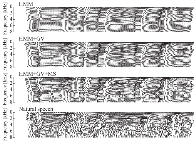
Fig. 11. An example of the spectrograms in HMM-based TTS.
