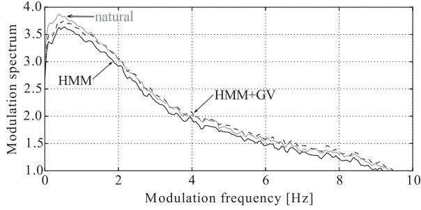
Fig. 4. Averaged MSs of log-F0 contours in HMM-based TTS. Note that the Nyquist frequency is 100 Hz similarly to the spectral parameters, but only < 10 Hz components are shown.
